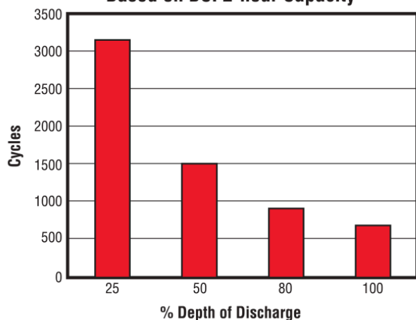
Cycle Life vs Depth of Discharge at +25°C (77°F) Based on BCI 2-hour Capacity
