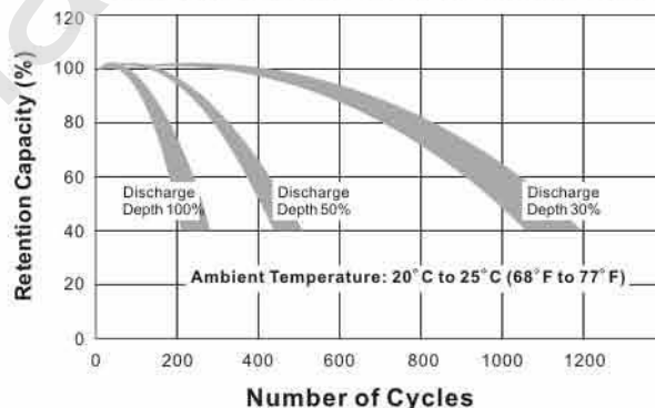
Life Characteristics in Cyclic Use
