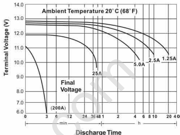
Discharge Characteristics
