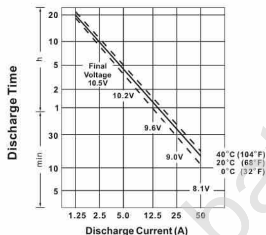
Discharge Time vs. Discharge Current
